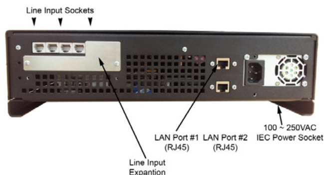
Total Recall LinX Neos: Rear View
